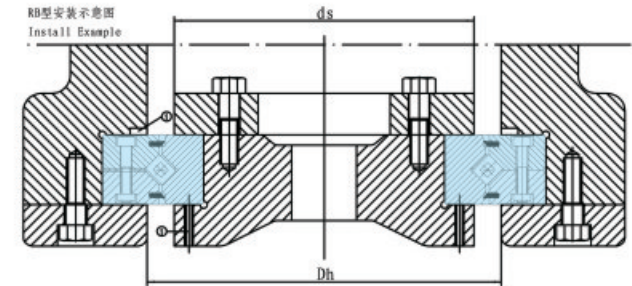
① 沟槽、螺纹退卸孔或用于拆卸用途的类似结构; Structures for Removing purposes;
